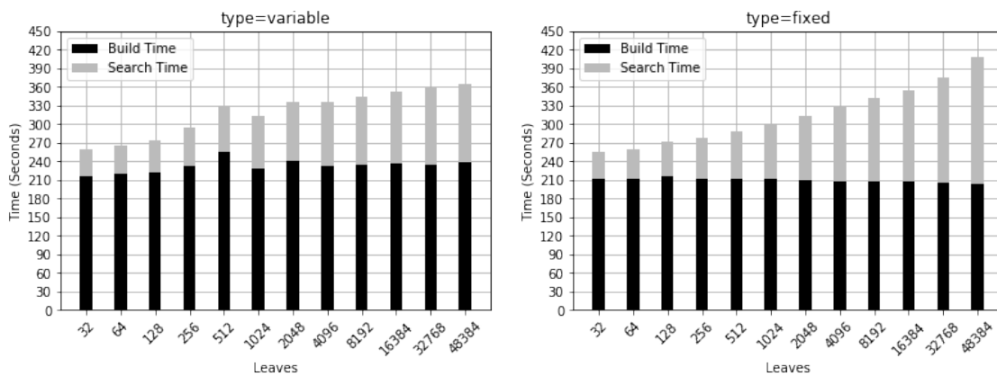
Figure 5. Time to search for t5 in a win7 tree.
